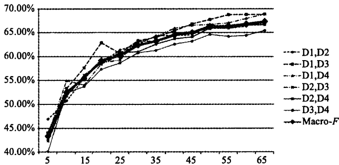
Fig.1 Learning curve of verbal model in “statement” frame
